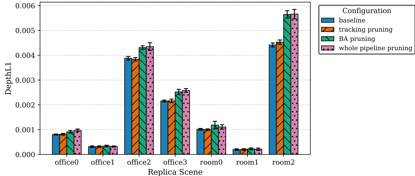
DepthL1 ( ↓ ) across Replica Scenes (Mean & Std Dev)
